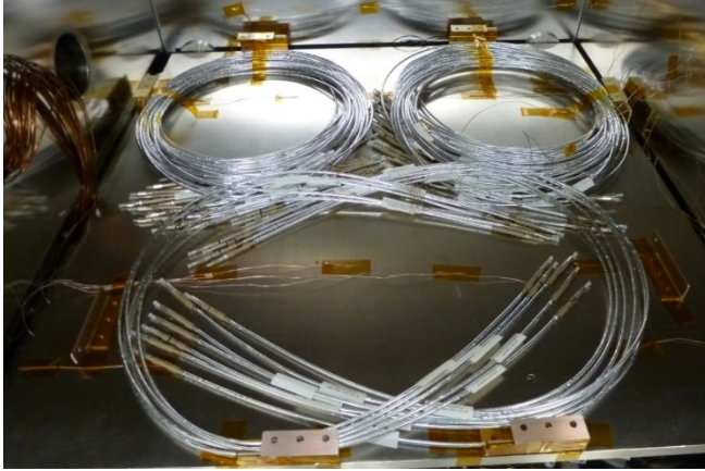
Figures 10 a & b: a) flight lot assemblies in the oven for thermal vacuum workmanship testing, b) fiber assembly ends on the TVAC oven thermal controlled plate with thermal couples attached to the assembly slip sleeves.
