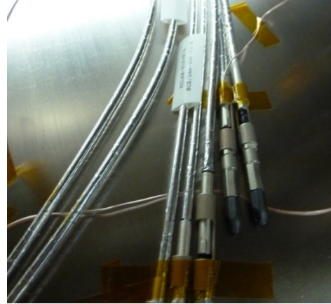
Figures 10 a & b: a) flight lot assemblies in the oven for thermal vacuum workmanship testing, b) fiber assembly ends on the TVAC oven thermal controlled plate with thermal couples attached to the assembly slip sleeves.
