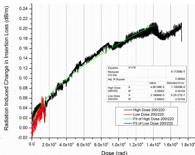
Figure 6a & 6b: Radiation induced loss data and analysis a: FV100110, b: FV200220
