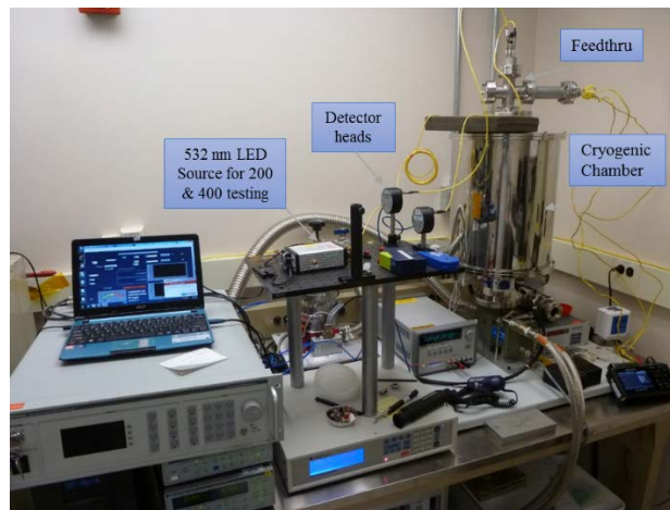
Figure 12: Experimental set up for cryogenic testing of the ATLAS ground support TVAC assemblies for usage at -115^{\circ}\text{C} .
