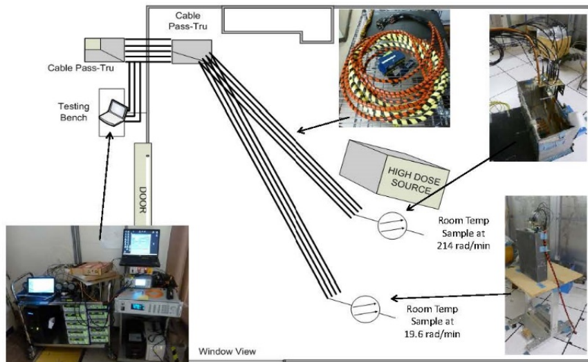
Figure 5: Radiation exposure data capture & testing set up
