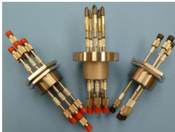
Figures 11 a & b: a) CarlisleIT LITEflightND cable terminated with FC and AVIM connectors by GSFC, b) optical fiber TVAC feedthrus as fabricated and designed for ATLAS by NASA GSFC
