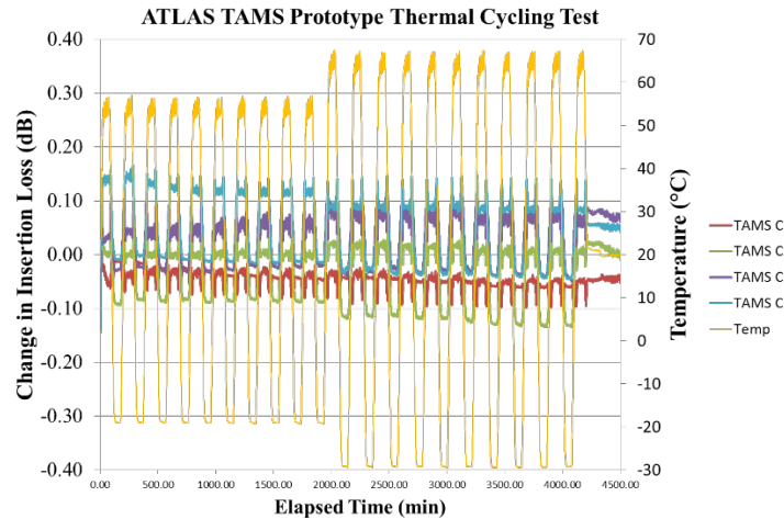
Figure 9: Thermal induced loss data for the quad array assembly prototype called "TAMS"
